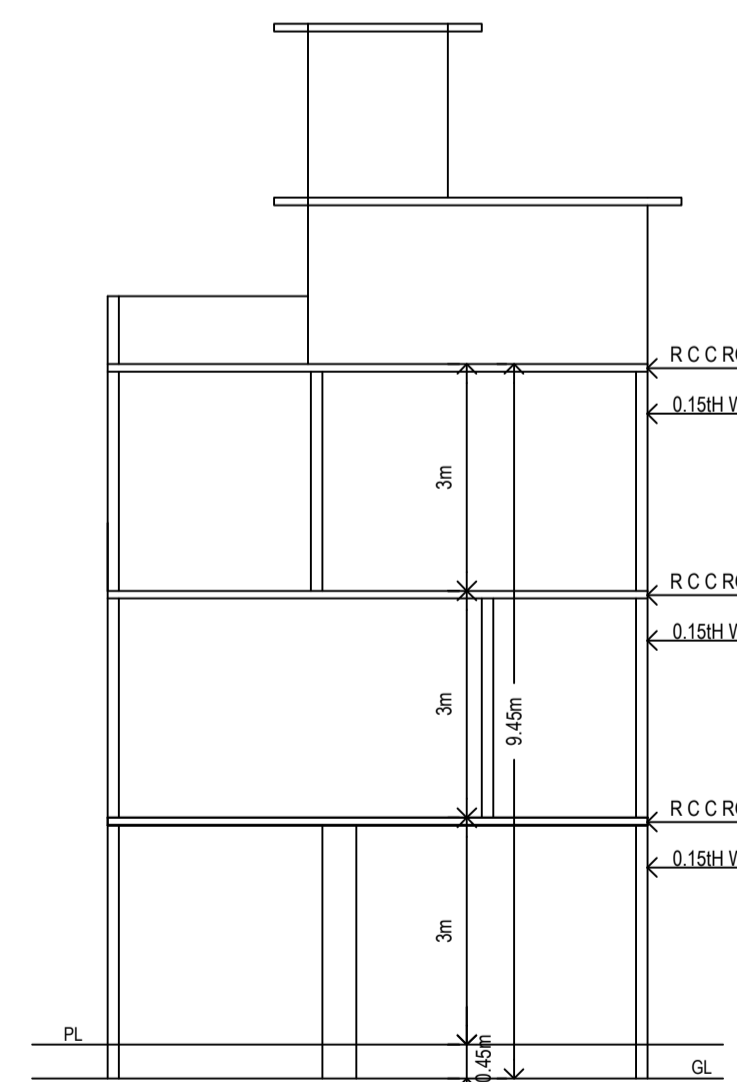
SECTION @ X-X
